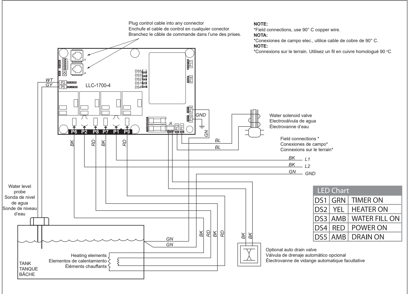
Figure 4A - Wiring Diagram Figura 4A - Diagrama de cableado Figure 4A - Schéma de câblage
